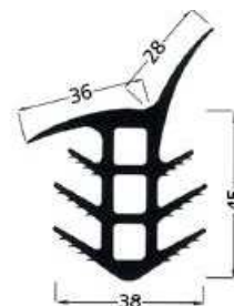
FA 15/3638 (for corner joints) Material: MIGUFLEX Joint width: 25 mm
