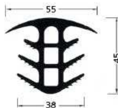
FA 15/5538 Material: MIGUFLEX Joint width: 25 mm
