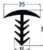
FA 135/35 Material: special PVC Joint width: 10 mm
